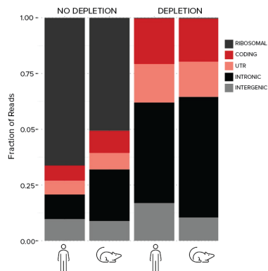
Figure 1: Genomic composition of libraries made with REALLY rNONE. 100ng of Universal total RNA from human or mouse (Agilent® Technologies) were used to make REALLY RNA-Seq libraries with or without the rNONE ribo-depletion module.
